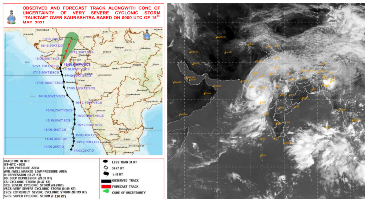
Figure: Observed and forecast track of cyclone and Satellite image as of 11:00 BST (Source: IMD)
