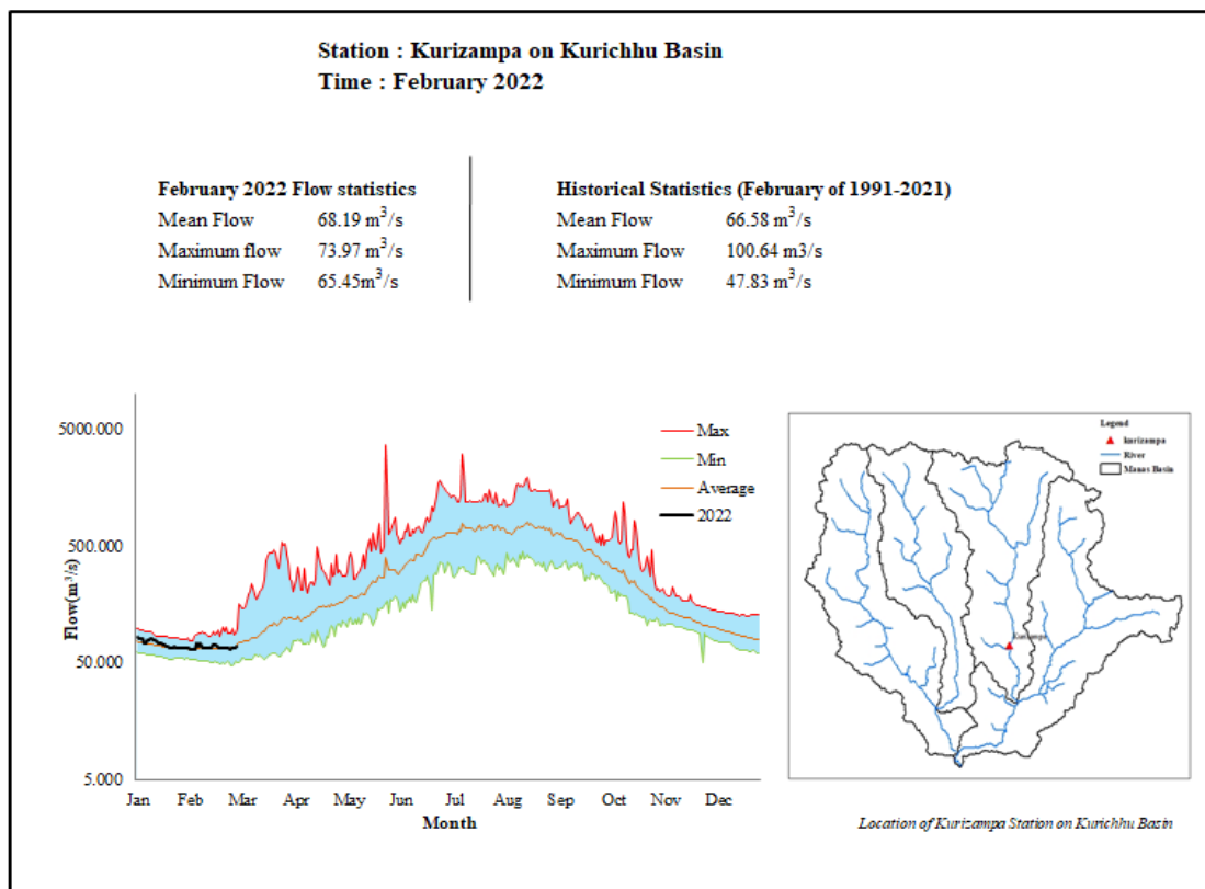
Figure 2 Daily flow status of February 2022 as compared to historical daily flow data of February months
