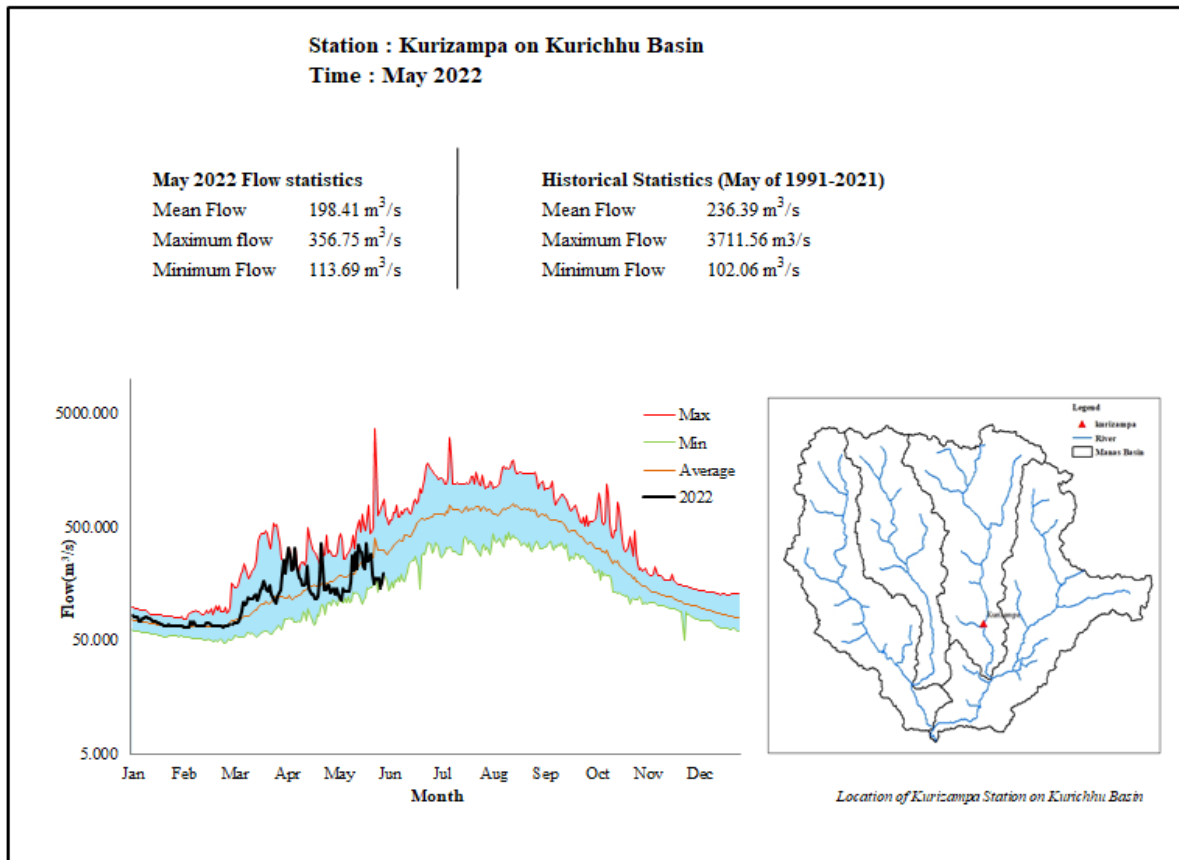
Figure 2 Daily flow status of May 2022 as compared to historical daily flow data of May months
