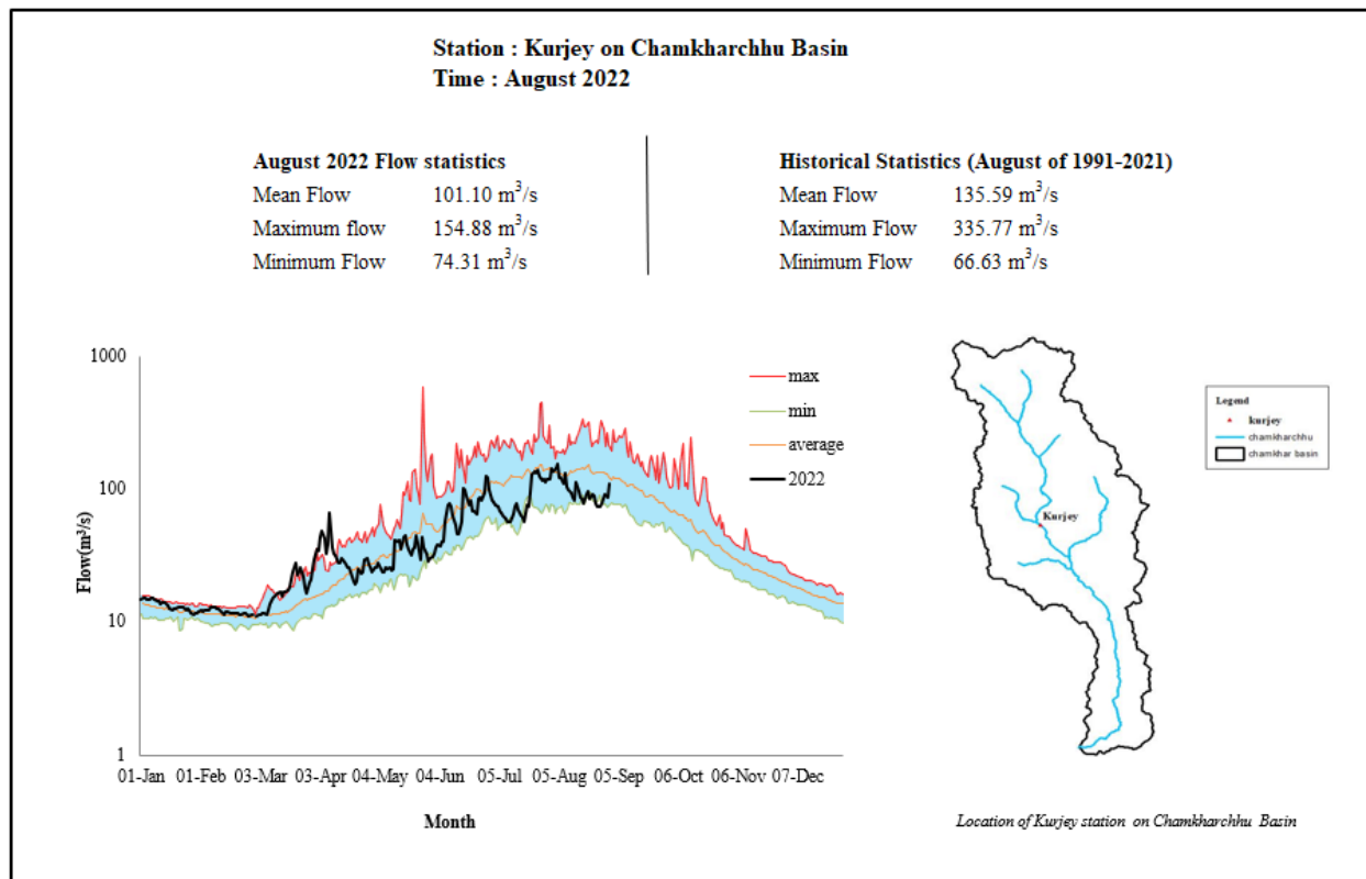
Figure 2 Daily flow status of August 2022 as compared to historical daily flow data of August months
