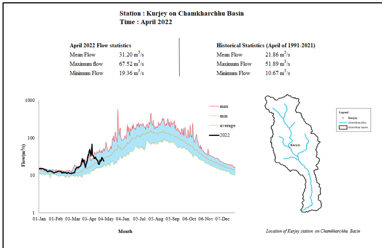
Figure 2 Daily flow status of April 2022 as compared to historical daily flow data of April months
