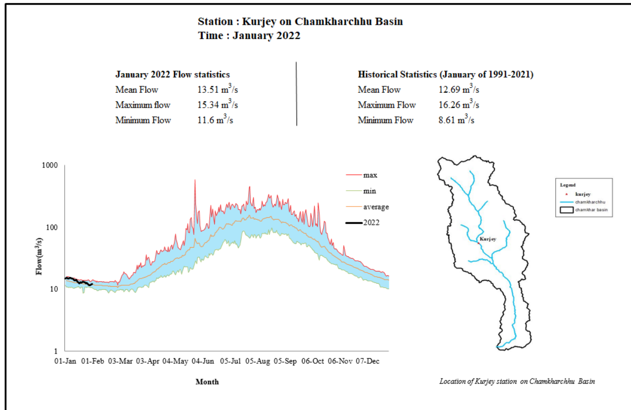
Figure 2 Daily flow status of January 2022 as compared to historical daily flow data of January months
