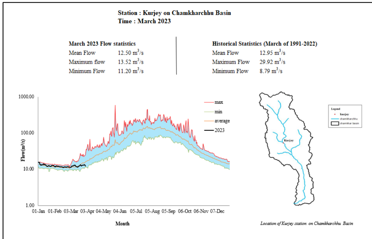
Figure 2 Daily flow status of March 2023 as compared to historical daily flow data of March months
