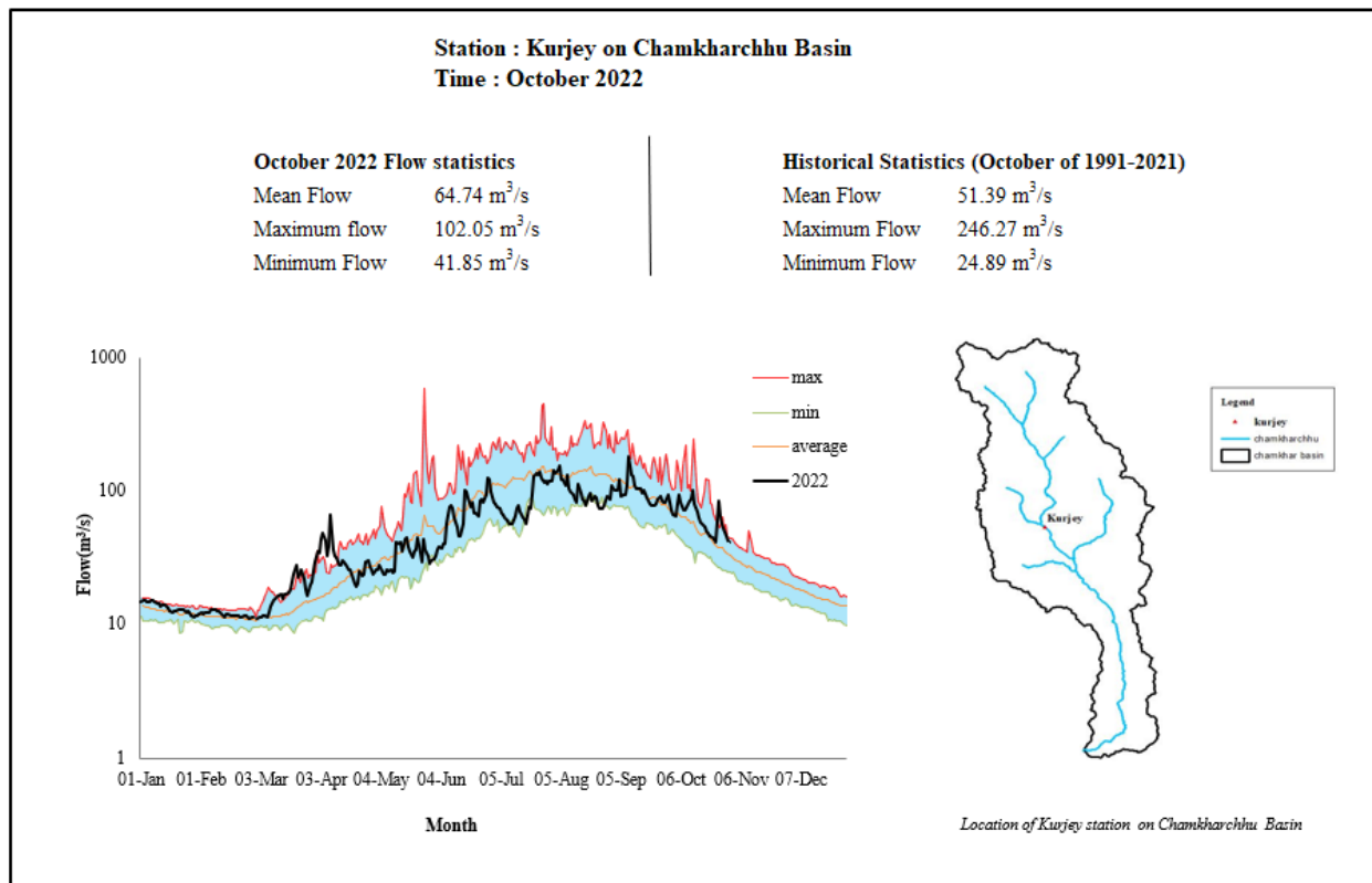
Figure 2 Daily flow status of October 2022 as compared to historical daily flow data of October months
