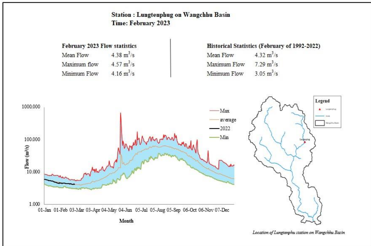
Figure 2 Daily flow status of February 2023 as compared to historical daily flow data of February months
