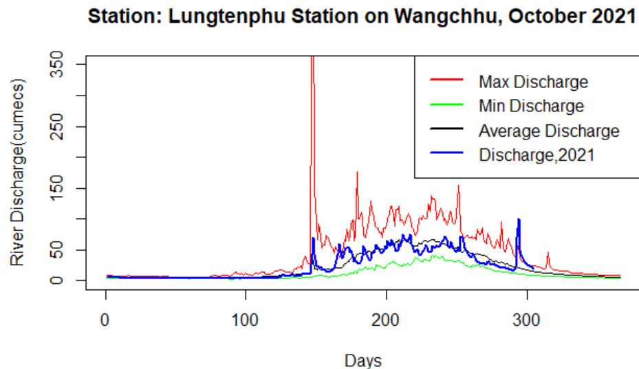
Figure 2 Daily flow status of October 2021 as compared to historical daily flow data of October months
