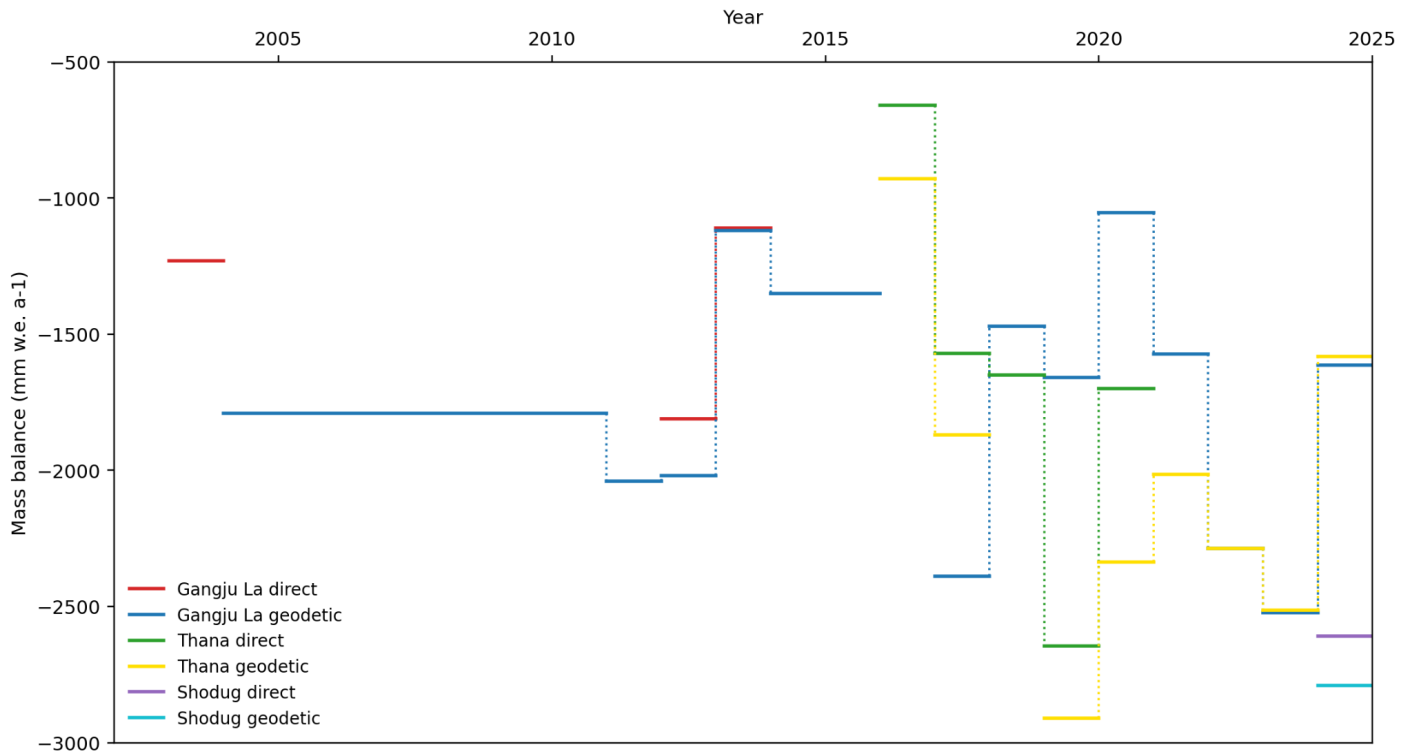
Figure 18: Mass balance of Three benchmark glaciers using different methods
