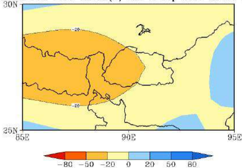
MMEM D&A Perc. Anom.(%) Jun to Sep 2017 Issued Apr
