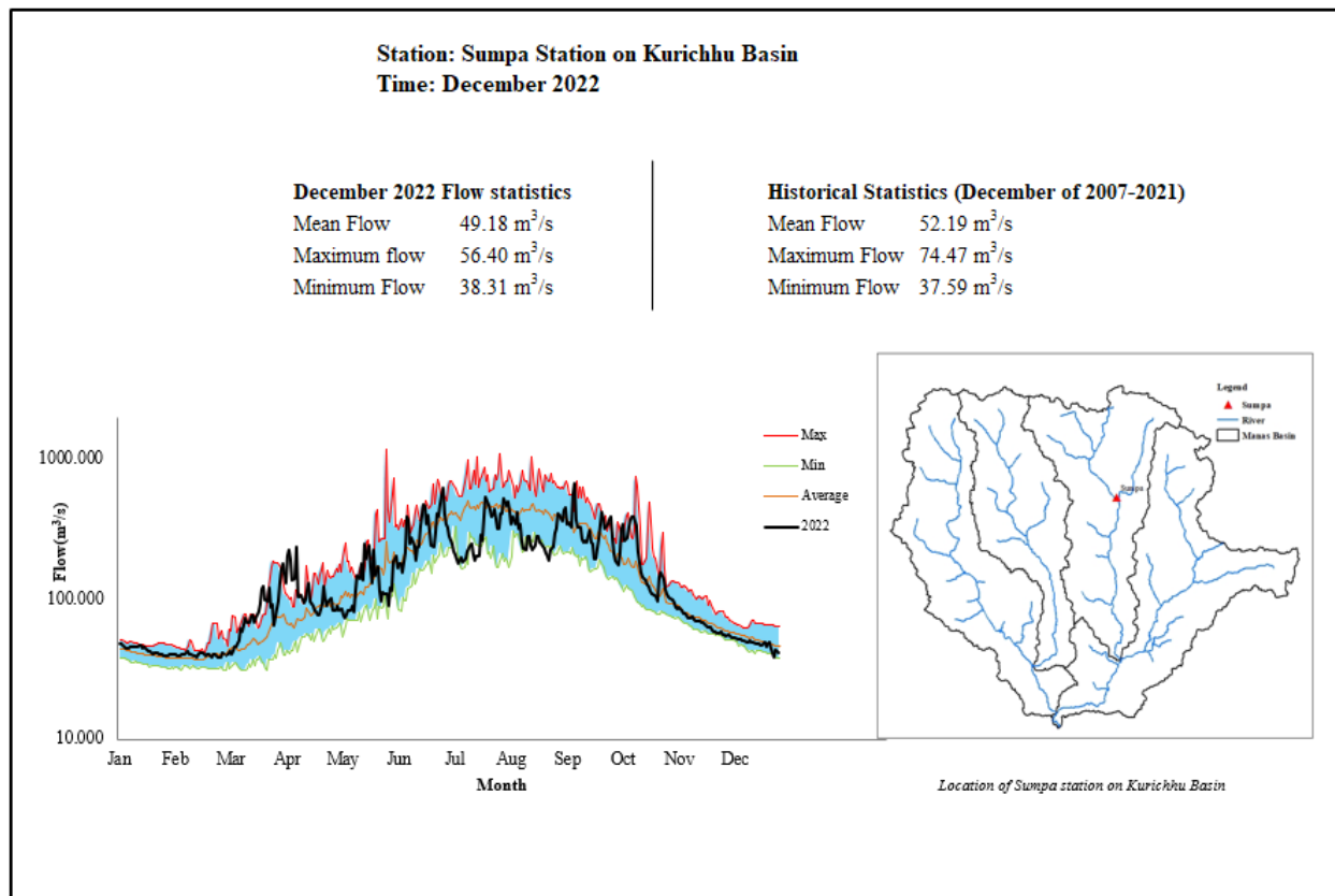
Figure 2 Daily flow status of December 2022 as compared to historical daily flow data of December months
