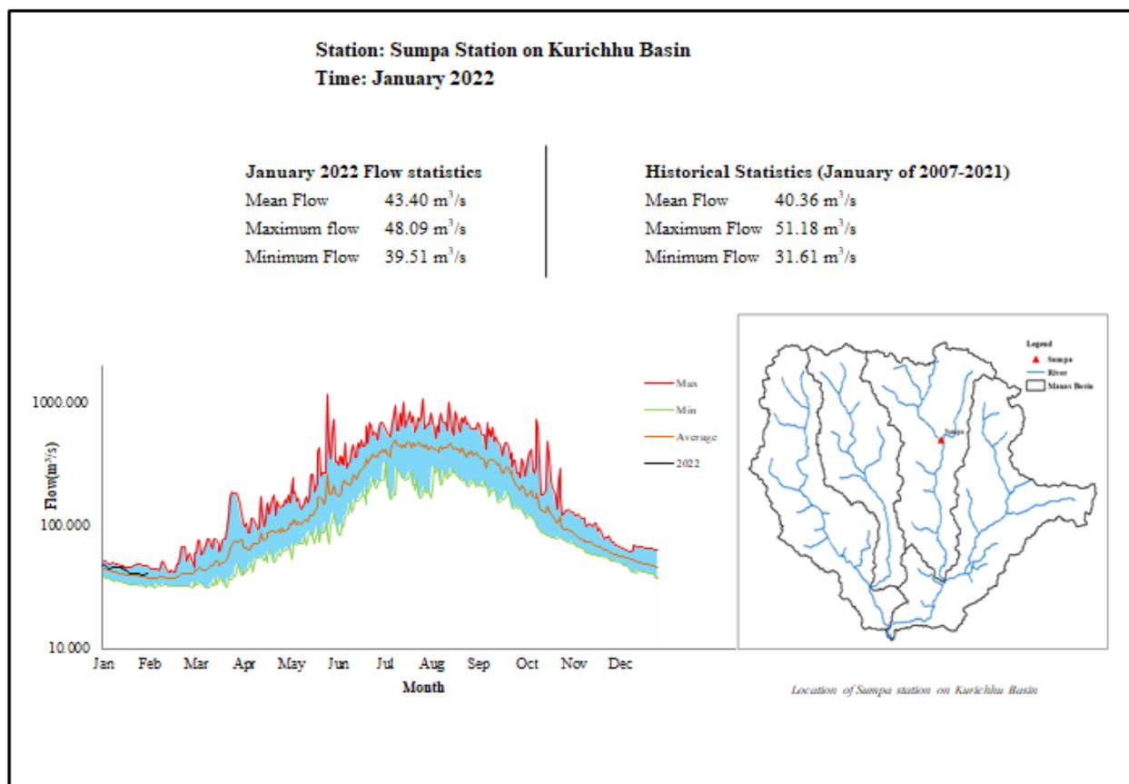
Figure 2 Daily flow status of January 2022 as compared to historical daily flow data of January months
