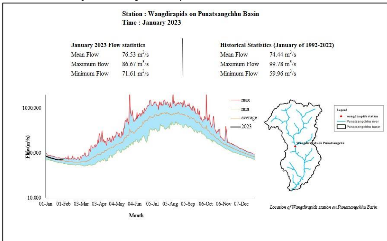
Figure 2 Daily flow status of January 2023 as compared to historical daily flow data of January months
