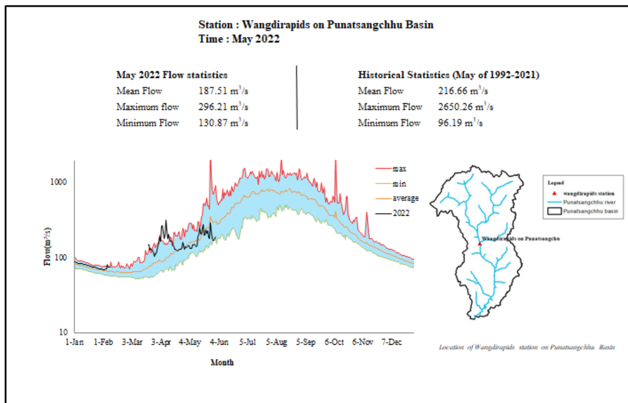
Figure 2 Daily flow status of May 2022 as compared to historical daily flow data of May months
