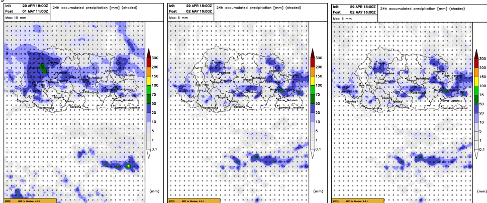
Figure: 24-hour total precipitation dated at 18 UTC, 29th April 2025
