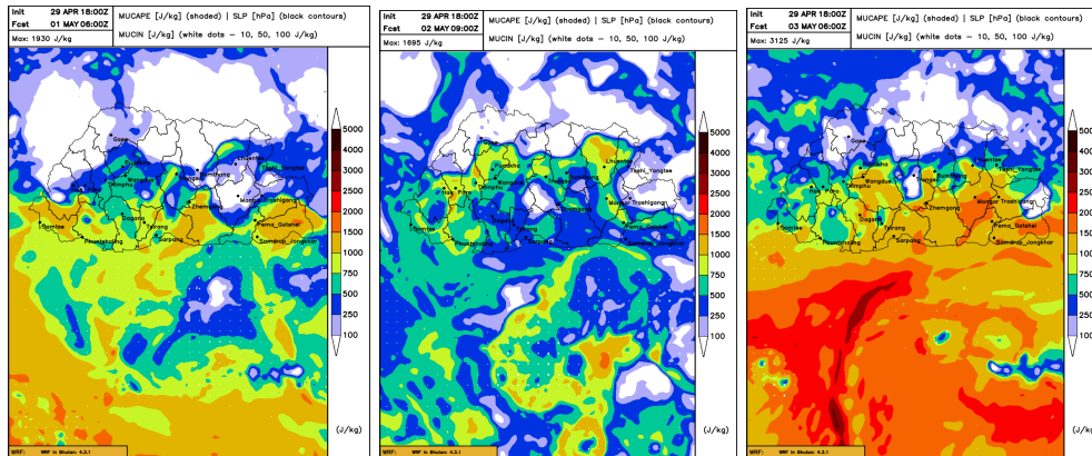
Figure: Mucape updated at 18 UTC, 29th April 2025
