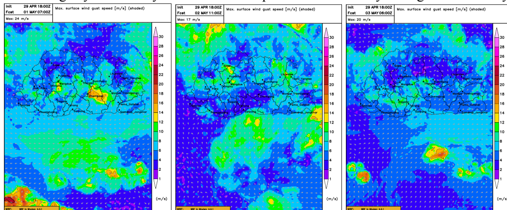
Figure: Wind Gust updated at 18 UTC, 29th April 2025
