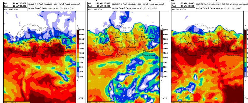
Figure: Mucape updated at 18 UTC, 20th May 2025
