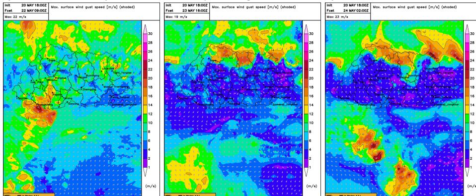
Figure: Wind Gust updated at 18 UTC, 20th May 2025
