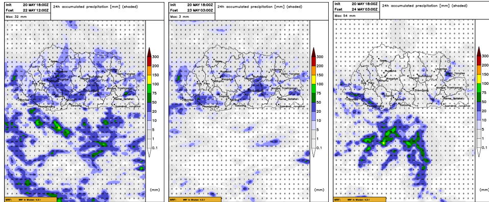
Figure: 24-hour total precipitation dated at 18 UTC, 20th May 2025
